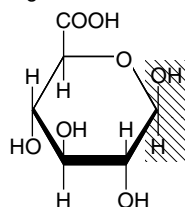
D-glucuronic acid
